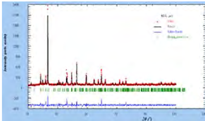
Fig. 1. Experimental X-ray powder diffraction pattern for with difference profile after Rietveld refinement.
