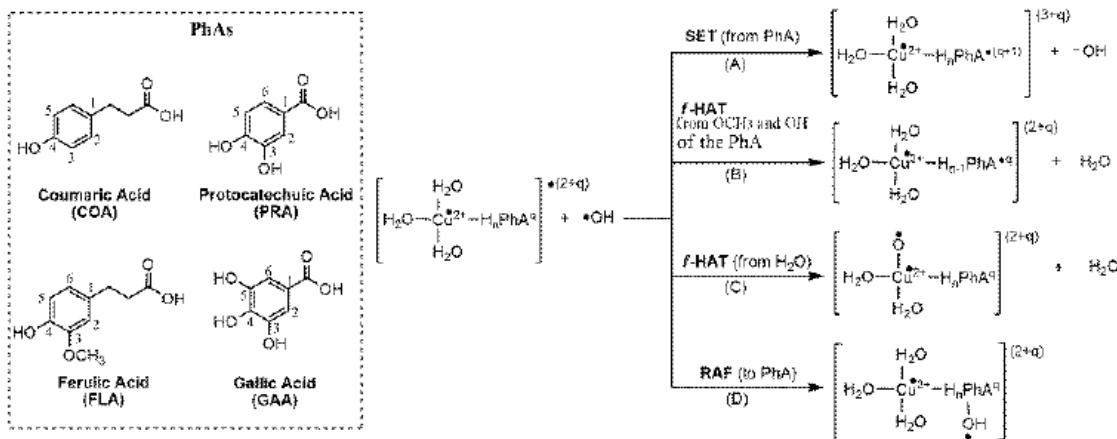
Scheme 1. (OIL-2) of PhAs-Cu(II).
