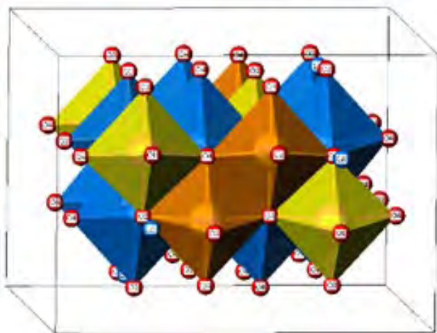
Fig. 2. \text{Li}_6\text{ZnZr}_3\text{O}_{10} . octahedron model. Blue Li atoms, green Zn atoms, and orange zirconium atoms.
